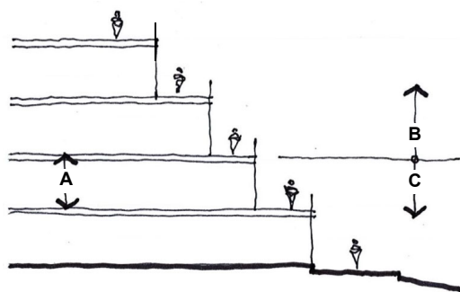
FIGURE 4814 Application of the visual privacy controls to roof terraces A - Second storey B - Refer to B3.5.4 C10 C - Refer to B3.5.4 C7
