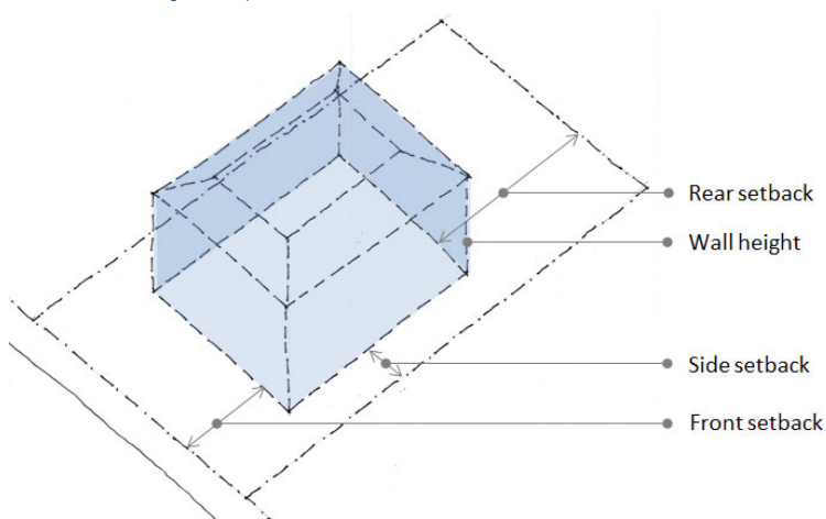
FIGURE 1 Building envelope
