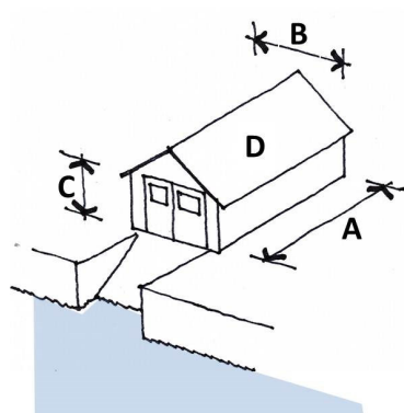
FIGURE 3431 Design considerations for boat sheds
